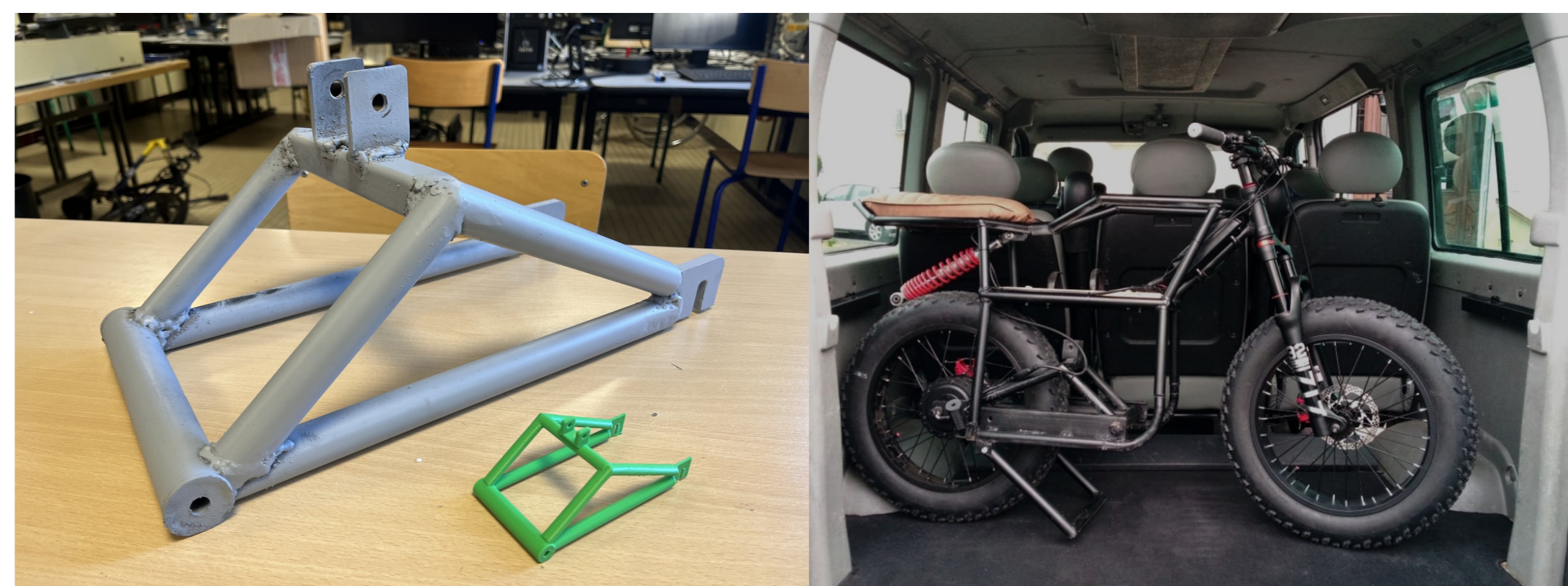
...nomenclature, welded chassis manufacturing, mechanical assembly, electrical wiring, procedure tests
